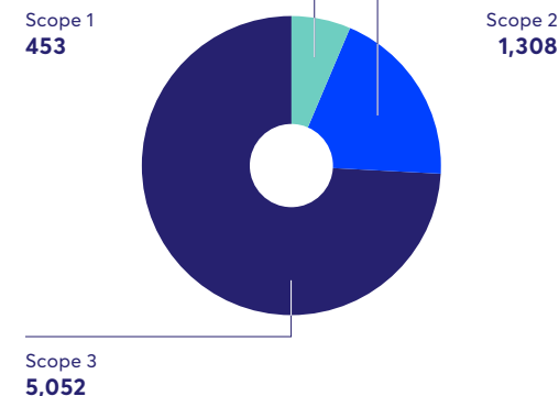
Emissions scope 1, 2 & 3
